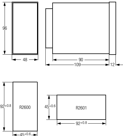
Bild 2, Case dimensions and panel cutout
